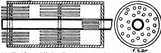
FIG. 308.—The "Loomis" Muffler. The exhaust enters the central tube at the right-hand end, passing out through slits shown in its side to the main chamber, where it is passed through a number of lengths of tubing. Leaving these it emerges to atmosphere through another set of tube lengths.
